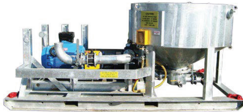
Dewatering Fish Tanks, Portable by QDS and capacities from 4,000l to 6,000l with up to 15,000l for permanent stations.
